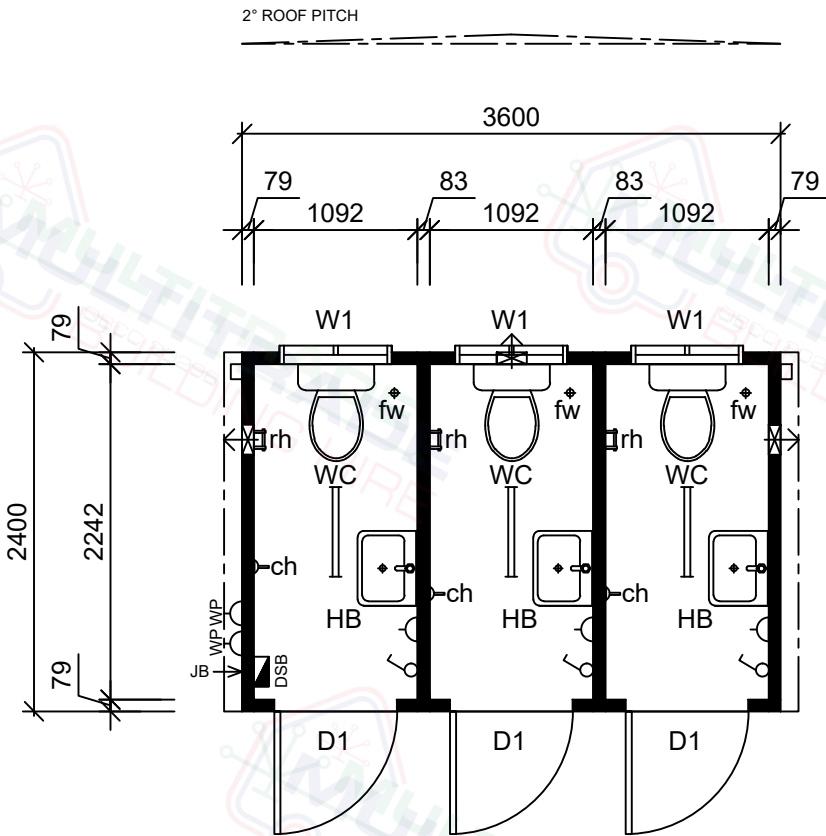
3.6x2.4m Toilet - Floor Plan
